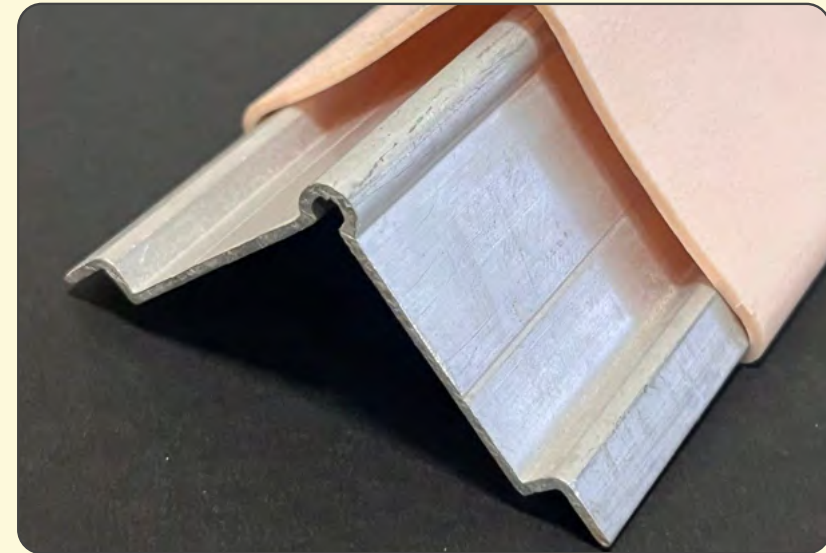
Aluminium Base with Pvc Insert and End cap
